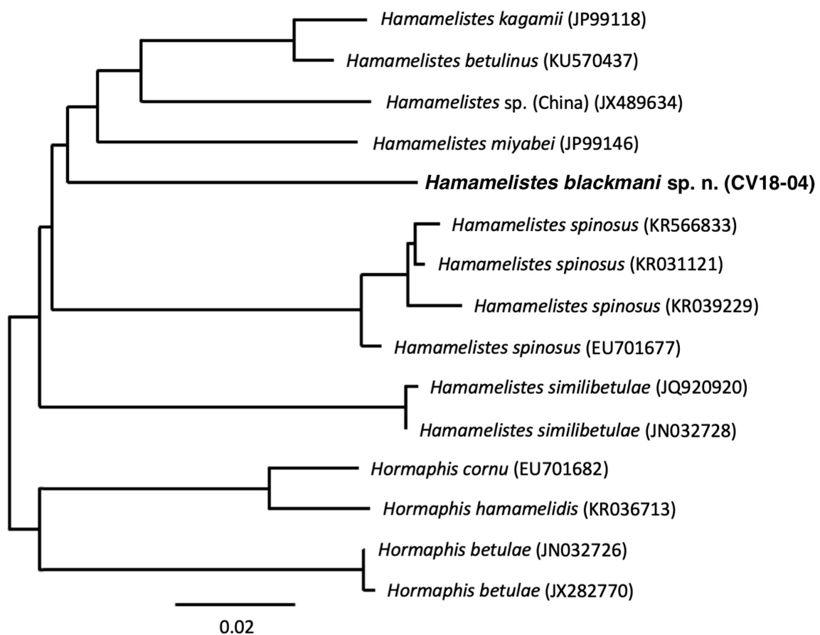
FIGURE 2. Neighbor-joining dendrogram from COI barcode DNA sequences, estimated under the K2P model of evolution. Hamamelistes blackmani sp. n. is shown in bold, clustered most closely to several Asian Hamamelistes species.
