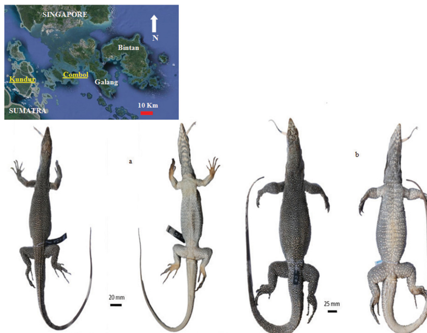
FIGURE 1. Dorsal and ventral sides of a: MZB.Lace.10293 ( Kundur ) and b: MZB.Lace.10294 ( Combol ). Inset: recorded localities of Varanus nebulosus in the Riau Archipelago, Indonesia. Photo: Evy Arida, Map: modified from Google Earth
