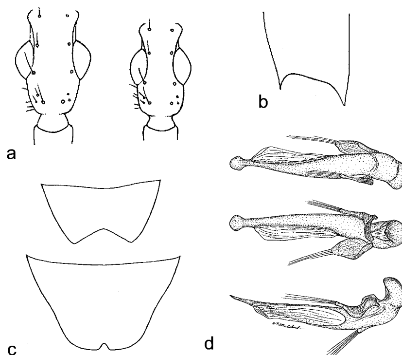
FIGURE 21. A. solanoi , dorsal aspect: a) head, male, female; b) apex of elytron; c) Sternum VI, male (top), female (bottom), ventral aspect; d) aedeagus, dorsal (top), ventral (middle), left lateral (bottom) aspects. Measures (mm): HL = 3.0; WE = 2.8; male SW = 4.4, female SW = 4.6; AL = 4.5.
