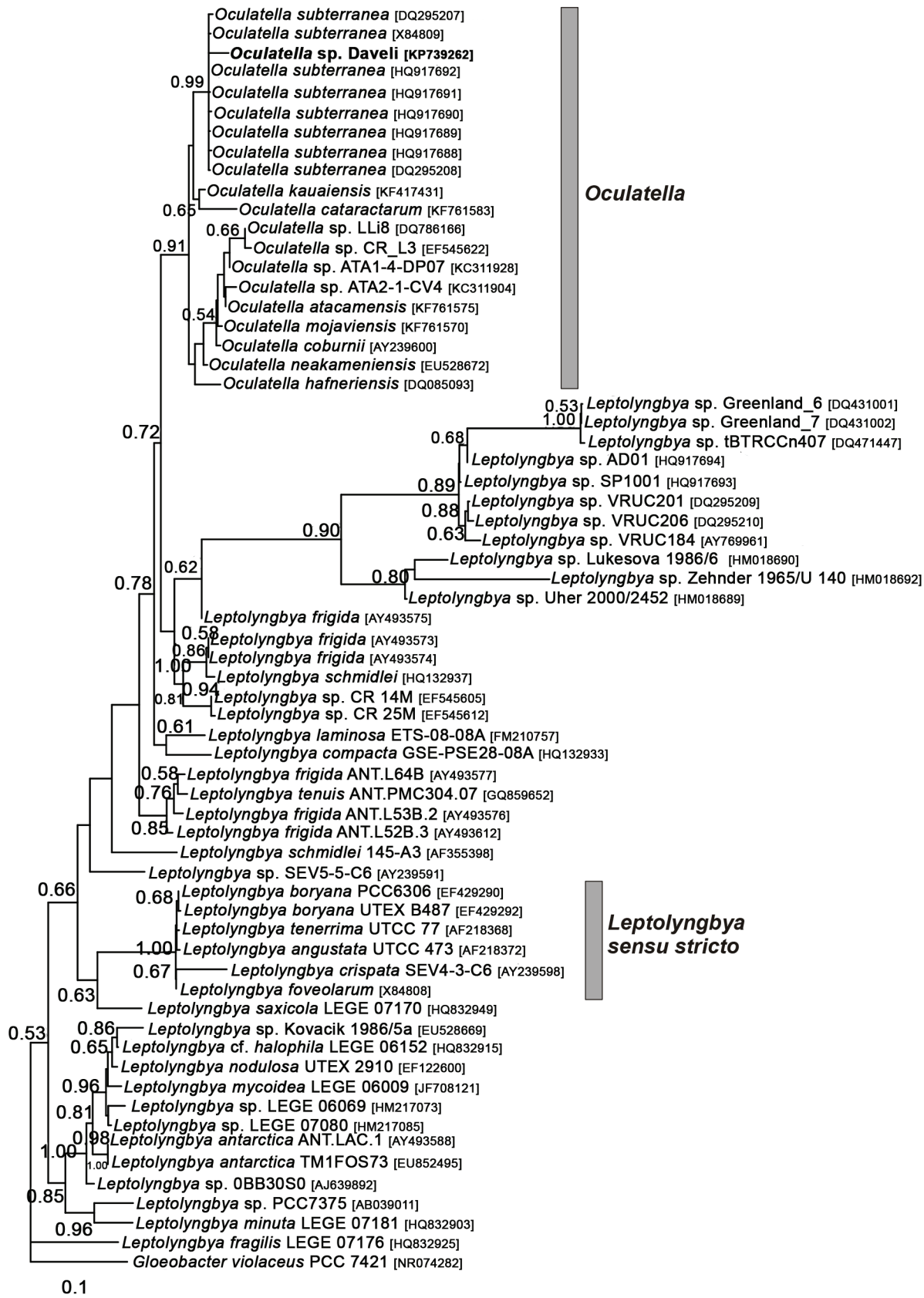
FIGURE S1. 50% majority-rule consensus tree of the Maximum Likelihood Analysis. Numbers at nodes correspond to the bootstrap values of the analysis (only values above 0.50 are provided). The Leptolyngbya sensu stricto clade (hosting the type species of the genus, L. boryana ) and the Ocumatella clade are indicated. Characters in bold indicate the taxon from Daveli Cave.
