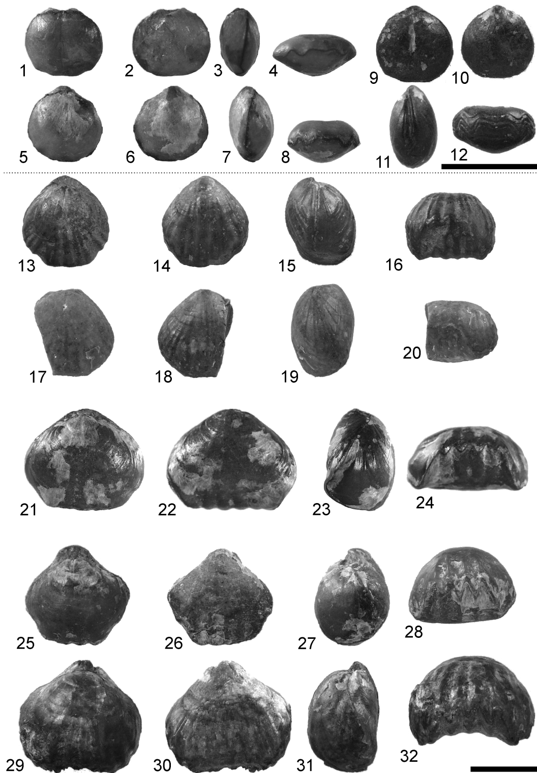
FIGURE 3. 1–12. Pseudomonticlairella varia Smirnova. 1–4. PMO 227.416, seep 13, dorsal, ventral, lateral, and anterior views. Specimen serially sectioned (Figure 4). 5–8. PMO 227.419, seep 7, dorsal, ventral, lateral, and anterior views. 9–12. PMO 227.418, seep 13, dorsal, ventral, lateral, and anterior views. 13–16. Ptilorhynchia mclachlani sp. nov. 13–16. PMO 224.876, seep 9, dorsal, ventral, lateral, and anterior views. 17–20, PMO 224.879, seep 9, dorsal, ventral, lateral, and anterior views. Specimen serially sectioned (Figure 5B). 21–24. PMO 227.431, seep 9, dorsal, ventral, lateral, and anterior views. Specimen serially sectioned (Figure 5A). 25–28. PMO 224.871, seep 9, dorsal, ventral, lateral, and anterior views. 29–32. Holotype, PMO 224.882, seep 9, dorsal, ventral, lateral, and anterior views. Dotted line delimits photographs at the same magnification. Scale bars = 1 cm.
