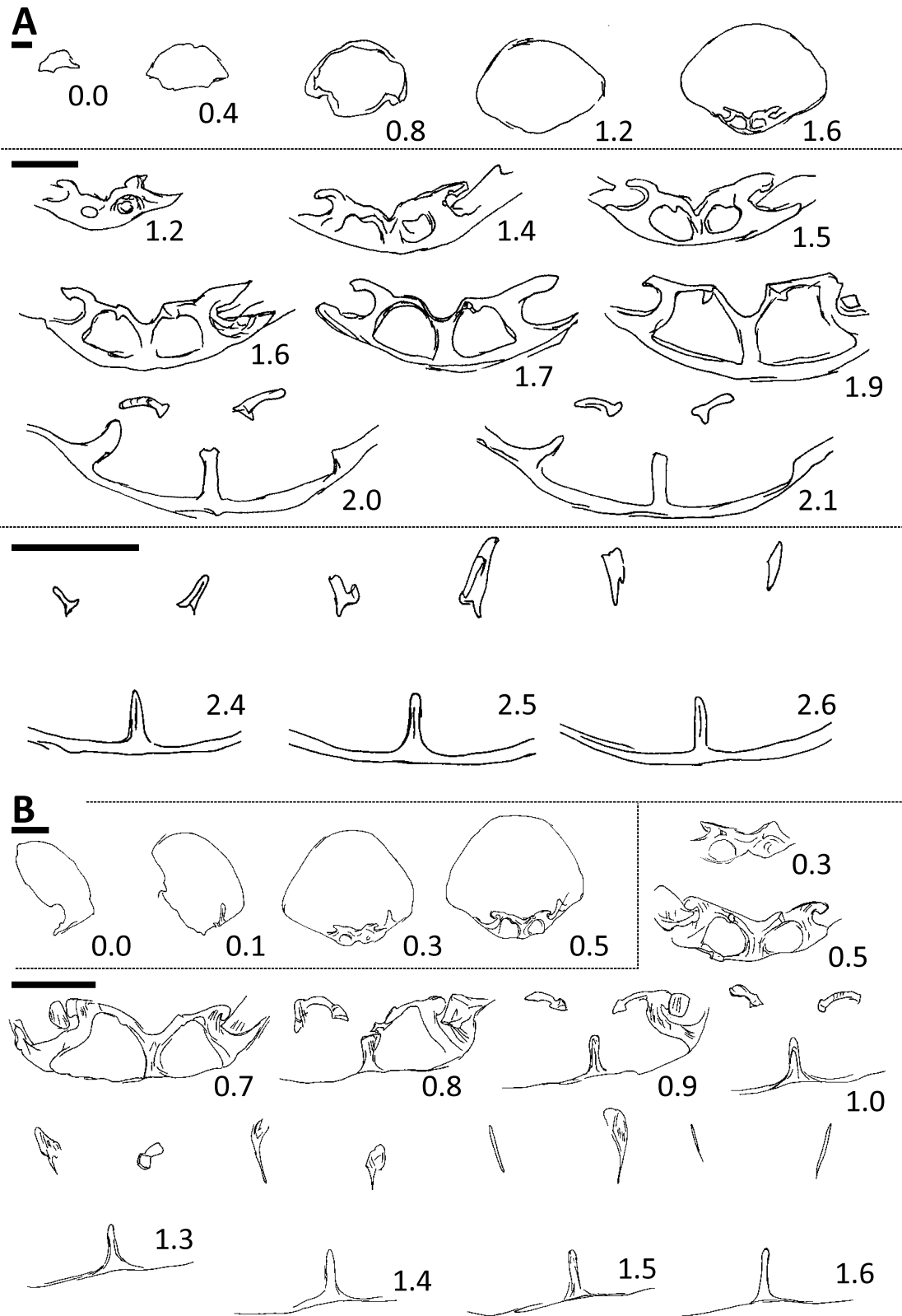
FIGURE 5. A and B, transverse serial sections from two specimens of Ptilorhynchia mclachlani sp. nov., seep 9. A) Specimen PMO 227.431, sections above third dotted line. Dotted lines delimit groups of sections drawn at the same magnification. Dimensions of specimen: L 15.3+; W 18.3; T 9.8 mm. Serial sections prepared perpendicular to maximum length of specimen; numbering of sections starts at 0.0 mm, the initial section through the specimen. B) Specimen PMO 224.879, sections below third dotted line. Dimensions of sectioned specimen: L 12.9; W 12.8+ ; T 9.0 mm. Serial sections prepared perpendicular to length of dorsal valve; numbering of sections starts at 0.0 mm, the initial section through the specimen. Scale bars = 1 mm.
