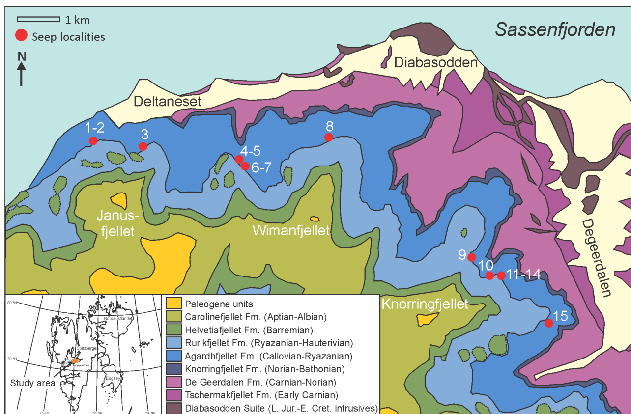
FIGURE 1. Geological map of the Late Jurassic–Early Cretaceous hydrocarbon seep carbonate localities, Spitsbergen (modified from Dallmann et al. 2001), with inset map of Svalbard indicating the study area.
