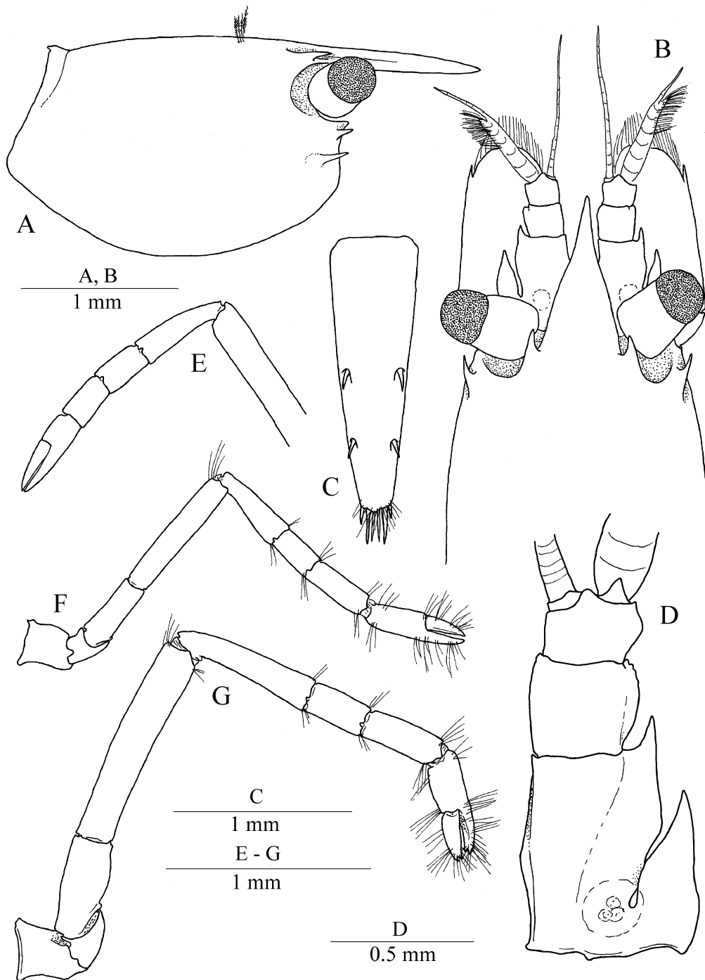
FIGURE 10. Alcyonohippolyte commensalis (Kemp, 1925) comb. nov., A–D, G, ovigerous female (pcl 2.5 mm); E, female (pcl 1.8 mm); F, ovigerous female (pcl 2.1 mm) (QM W33475): A, B, carapace; C, telson; D, antennule; E–G, pereopod II.
